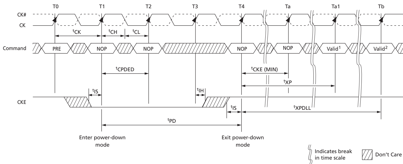
Figure 95: Precharge Power-Down (Slow-Exit Mode) Entry and Exit
