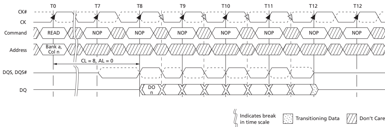
Figure 64: READ Latency
