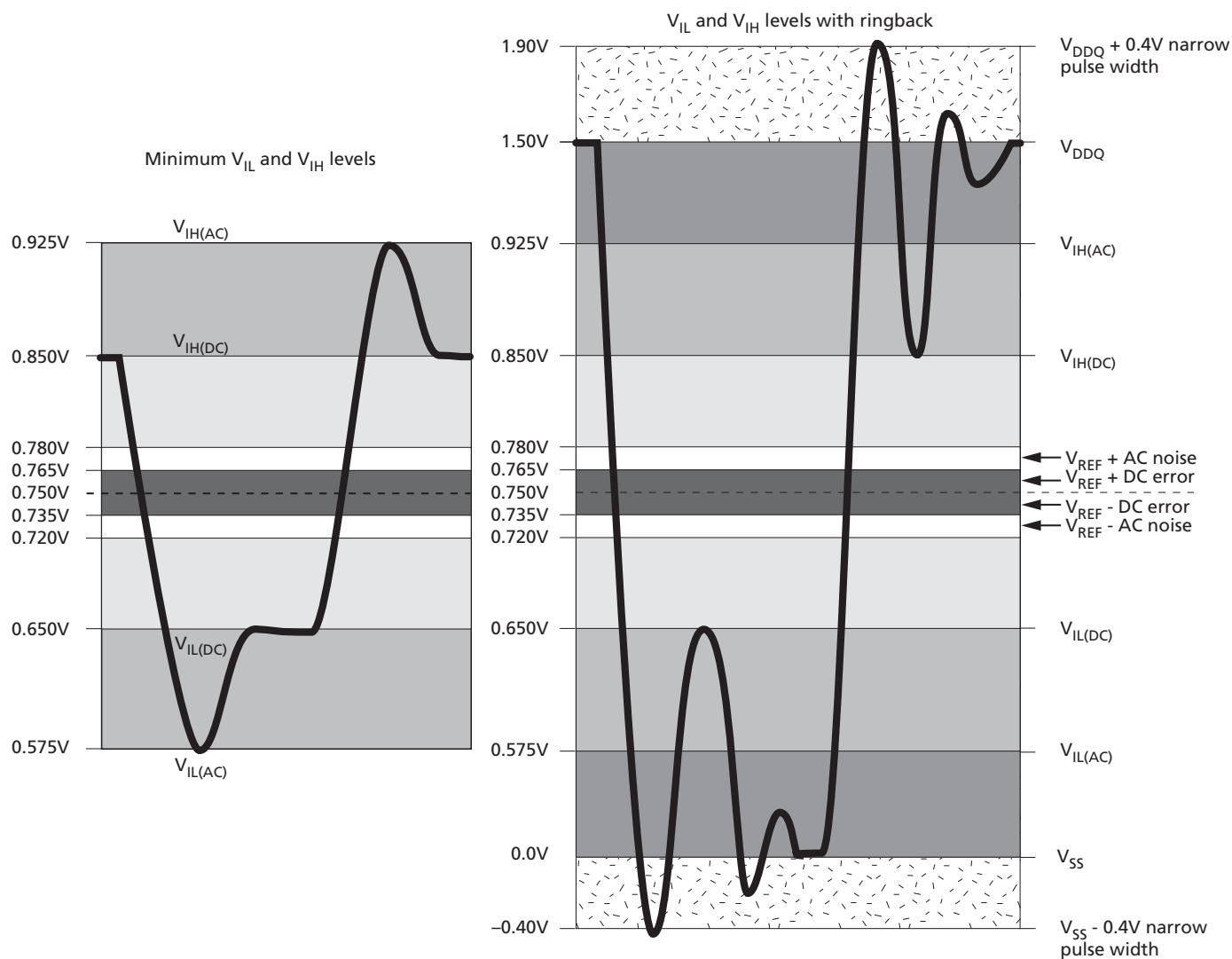
Figure 11: Input Signal
