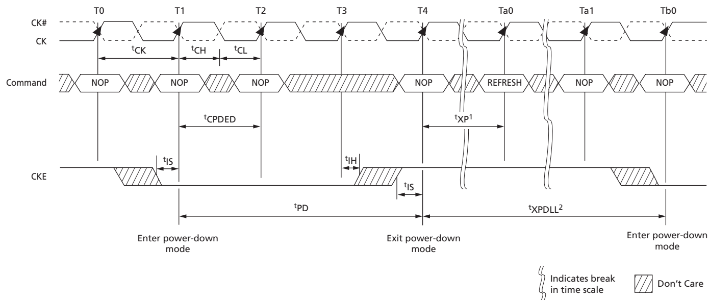
Figure 103: Power-Down Exit to Refresh to Power-Down Entry
