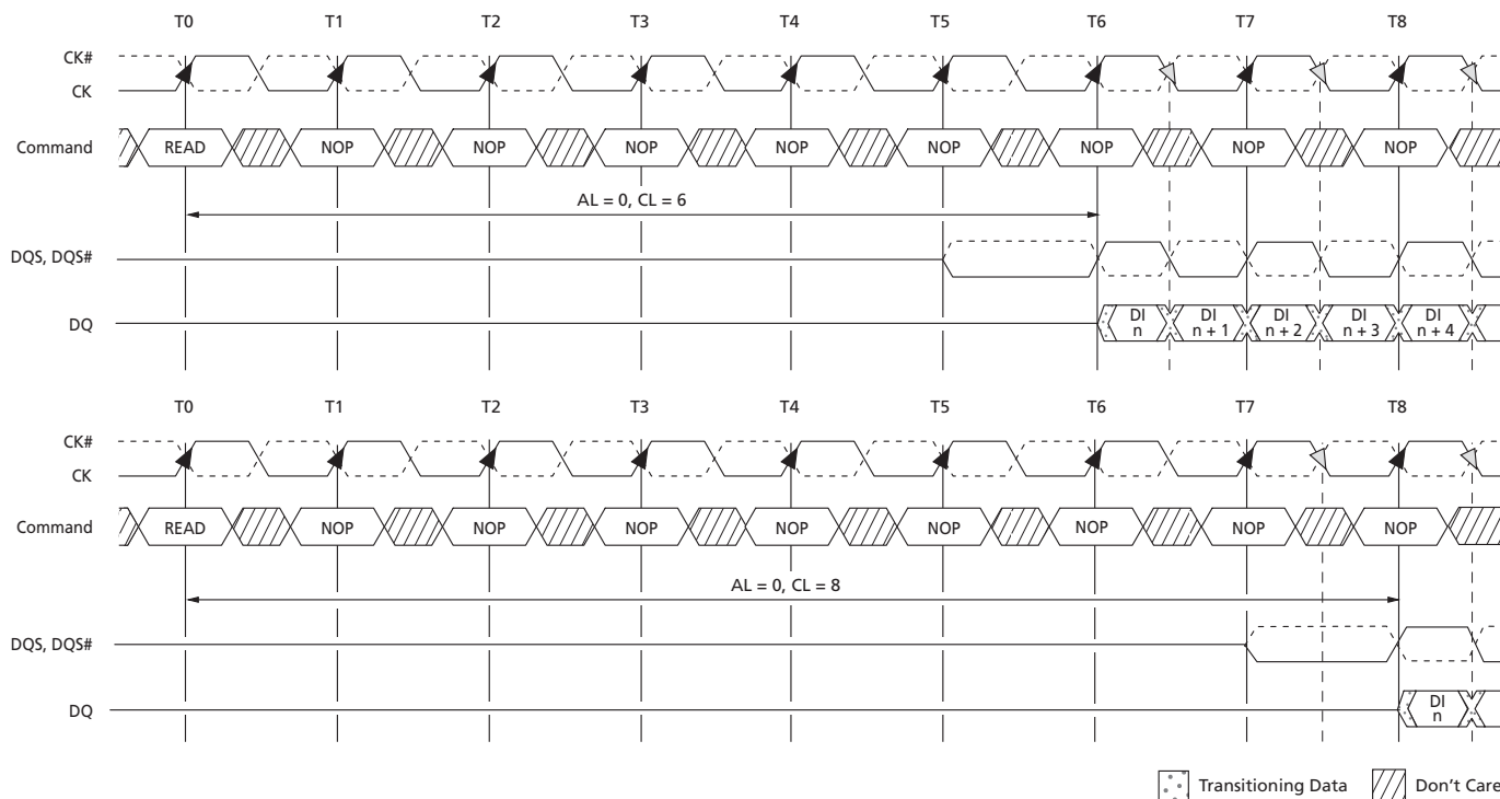
Figure 50: READ Latency
