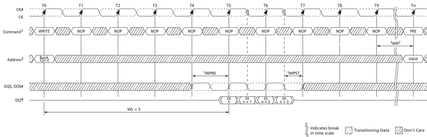
Figure 90: WRITE (BC4 OTF) to PRECHARGE
