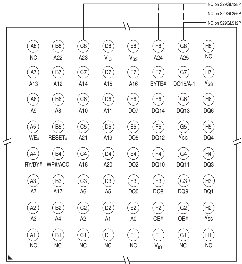
Top View, Balls Facing Down
