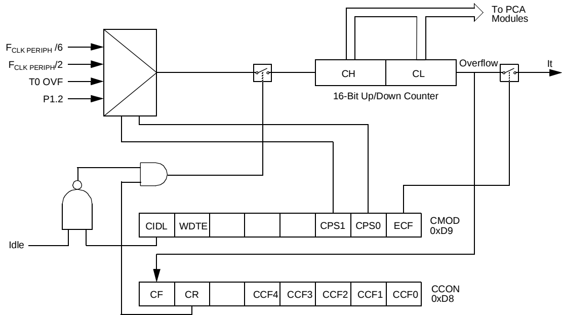
Figure 8. PCA Timer/Counter
