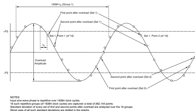
Figure 33. Overload Recovery
