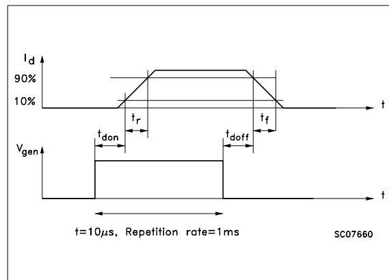
Figure 6: Waveforms
