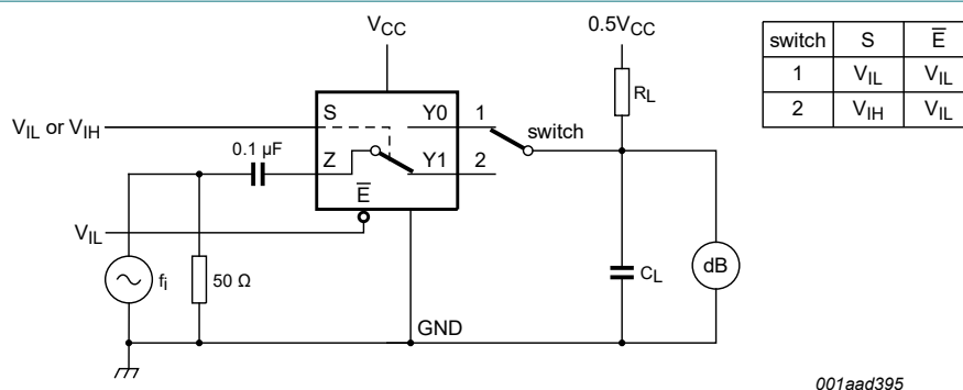
Fig. 16. Test circuit for measuring the frequency response when switch is in ON-state
