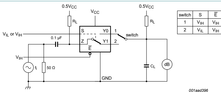
Fig. 17. Test circuit for measuring isolation (OFF-state)
