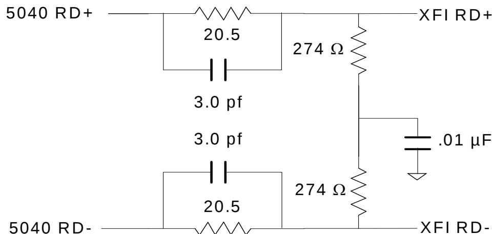
Figure 17. RD Pre-Emphasis Circuit
