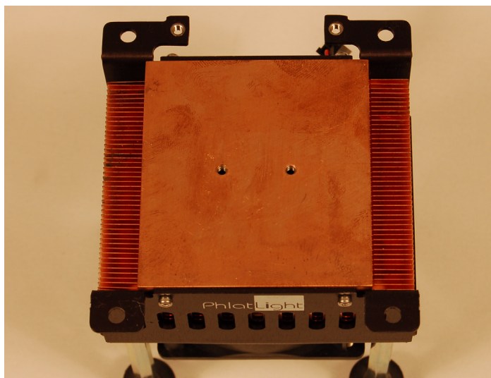
Figure 10: Pre-drilled holes
