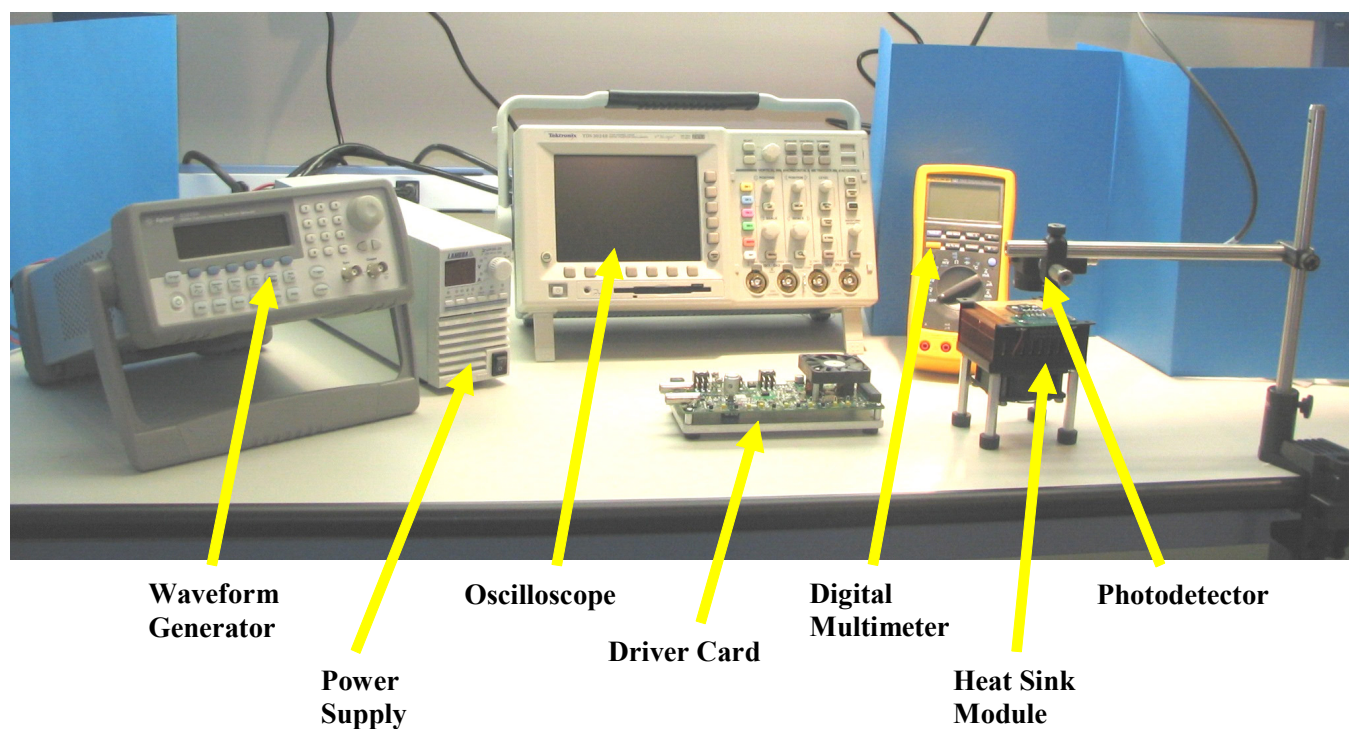
Figure 16: Equipment set up for PhlatLight™ evaluation (example)
