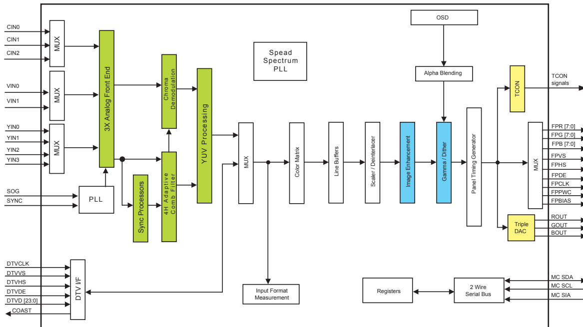
TW8806 Block Diagram
