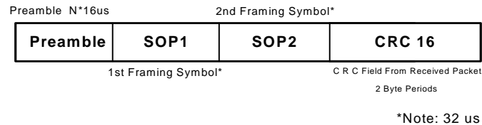
Figure 3. Example ACK Packet Format
