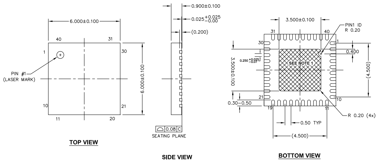
Figure 11. 40-pin QFN (6 × 6 × 0.90 mm) 3.5 × 3.5 E-Pad (Sawn) Package Outline, 001-44328
