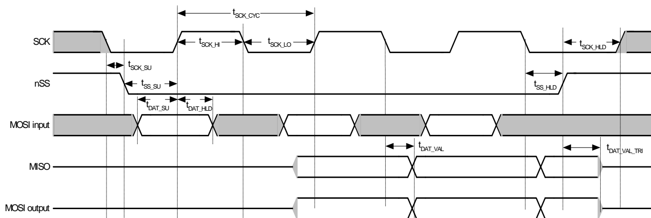
Figure 8. SPI Timing
