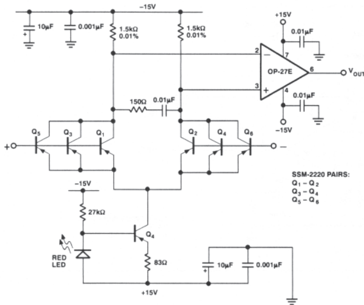
FIGURE 1a: Super Low Noise Amplifier
