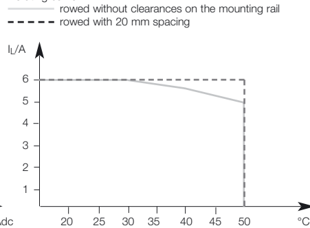
Derating curve
