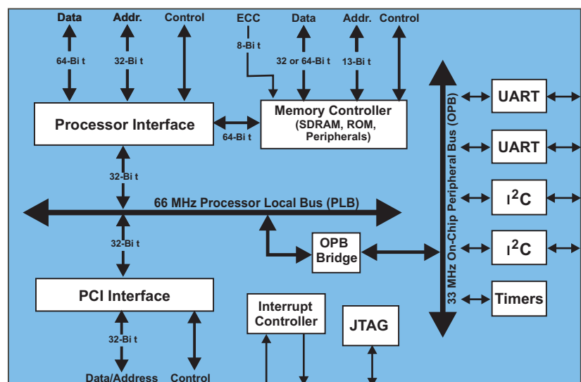
CPC700 Block Diagram
