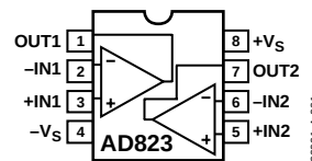
Figure 1. 8-Lead PDIP and SOIC
