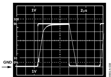
Figure 38. AD823 Input Response: Response with R_P = 0 , V_{IN} from 0 to V_S
