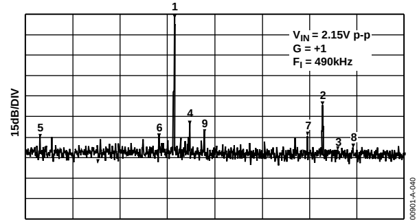
Figure 41. FFT of AD1672 Output Driven by AD823
