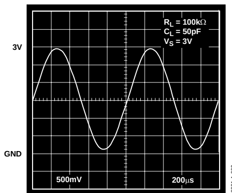
Figure 2. Output Swing, V_S = 3 V, G = +1
