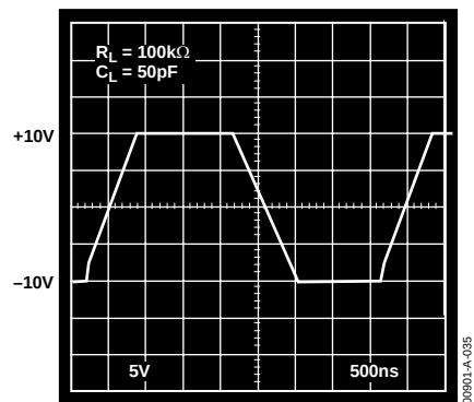
Figure 35. Pulse Response, V_S = \pm 15V , G = +1
