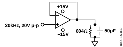
Figure 32. Output Swing, V_S = \pm 15\text{ V} , G = +1
