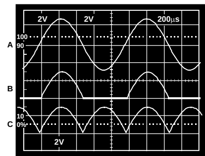
Figure 46. Single-Supply Half-Wave and Full-Wave Rectifier
