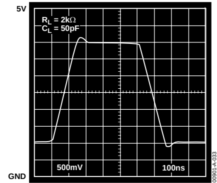
Figure 33. Pulse Response, V_S = 5\text{ V} , G = +1
