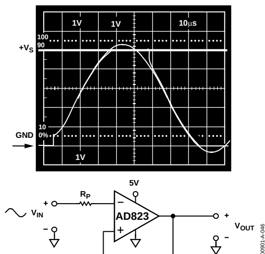
Figure 39. AD823 Input Response: V_{IN} = 0 to +V_S + 200 mV, V_{OUT} = 0 to +V_S , R_P = 49.9 k \Omega
