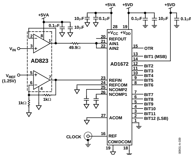
Figure 40. AD823 Driving Input and Reference of the AD1672, a 12-Bit, 3 MSPS ADC
