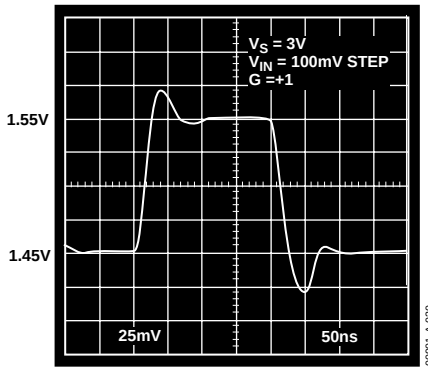
Figure 30. Pulse Response, V_S = 3\text{ V} , G = +1
