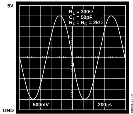
Figure 29. Output Swing, V_S = 5\text{ V} , G = -1
