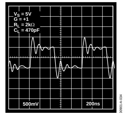
Figure 34. Pulse Response, V_S = 5\text{ V} , G = +1 , C_L = 470\text{ pF}
