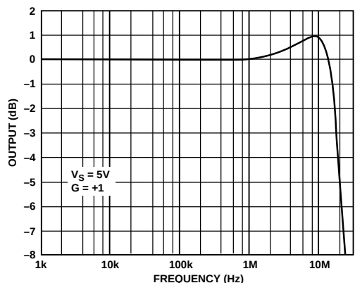
Figure 3. Small Signal Bandwidth, G = +1
