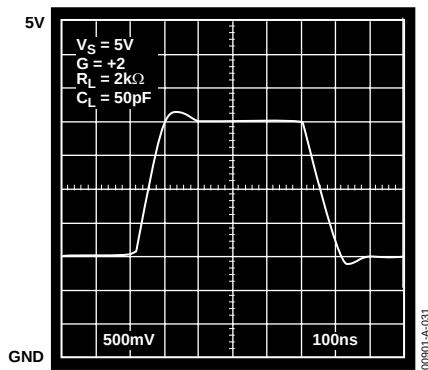
Figure 31. Pulse Response, V_S = 5\text{ V} , G = +2
