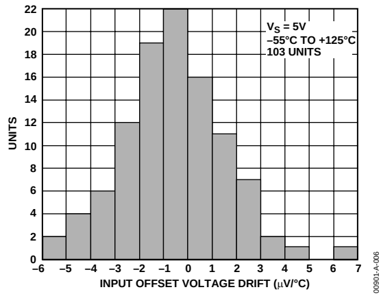
Figure 6. Typical Distribution of Input Offset Voltage Drift
