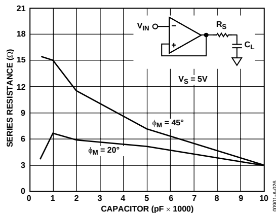
Figure 26. Capacitive Load vs. Series Resistance
