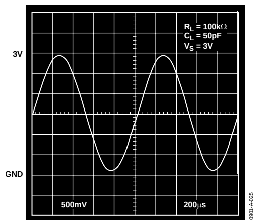
Figure 25. Output Swing, V_S = 3V , G = +1
