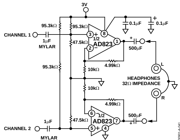
Figure 42. 3 V Single-Supply Stereo Headphone Driver
