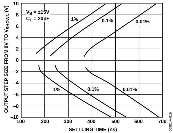
Figure 19. Inverter Settling Time vs. Output Step Size
