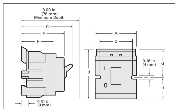
Shaft Mounted 3LD2 Handle Cutout
