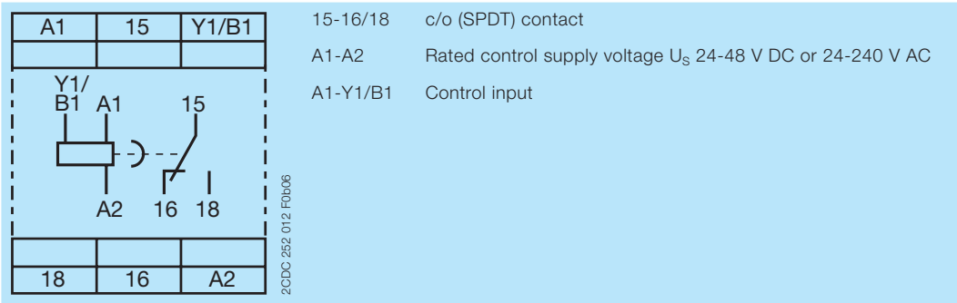
Connection diagram
