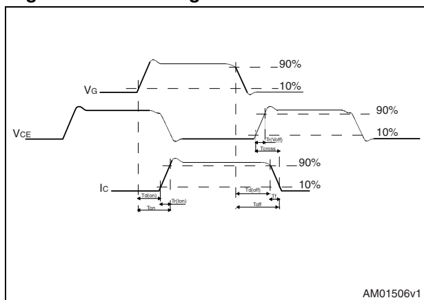
Figure 21. Switching waveform
