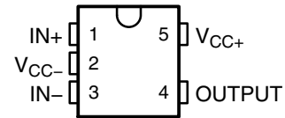
LPV321 . . . DBV OR DCK PACKAGE (TOP VIEW)
