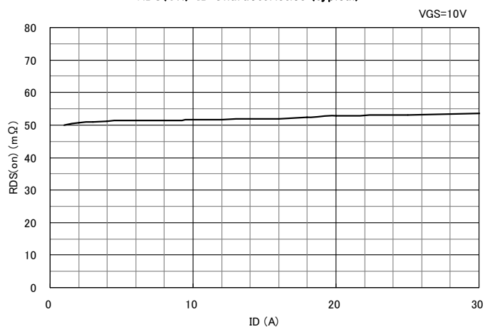
RDS(ON)-ID Characteristics (typical)
