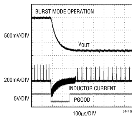
V_{OUT(MAX)} to V_{OUT(MIN)} Transition
