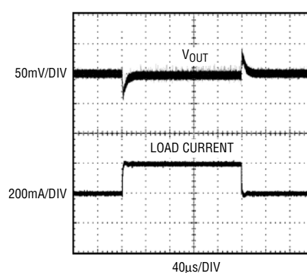
Load Step (200mA to 400mA)
