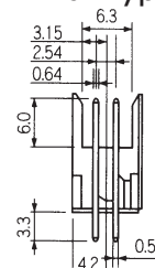
Type 04 - Straight solder dip terminal
