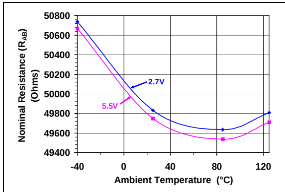
FIGURE 2-41: 50 kΩ – Nominal Resistance ( R_{AB} ) (Ω) vs. Ambient Temperature and V_{DD} .
