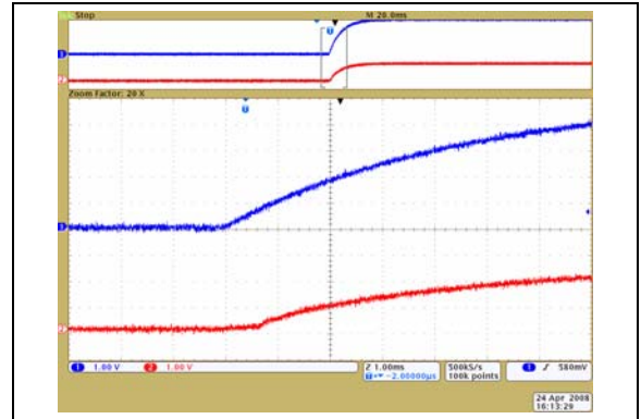
FIGURE 2-50: 50 k \Omega – Low-Voltage Increment Wiper Settling Time ( V_{DD} = 2.7\text{V} ) (1 \mu\text{s}/\text{Div} ).
