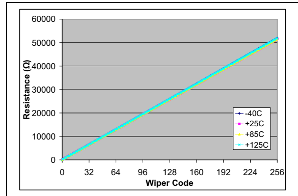
FIGURE 2-42: 50 kΩ – R_{WB} (Ω) vs. Wiper Setting and Ambient Temperature ( V_{DD} = 5.5\text{V} , I_W = 90\text{ }\mu\text{A} ).
