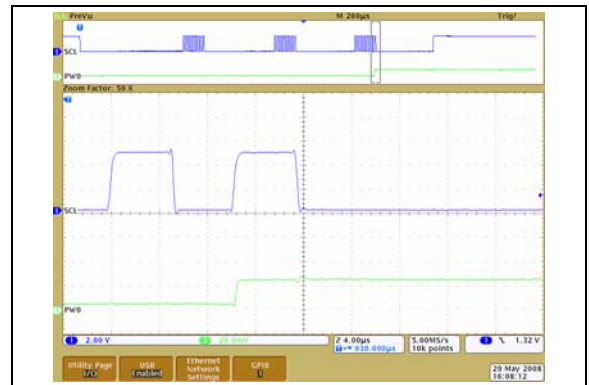
FIGURE 2-51: 50 k \Omega – Low-Voltage Increment Wiper Settling Time ( V_{DD} = 5.5\text{V} ) (1 \mu\text{s}/\text{Div} ).
