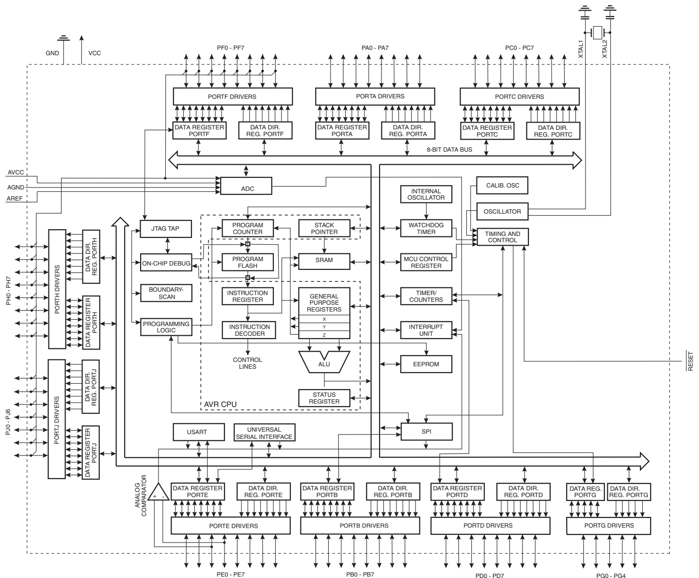
Figure 2-1. Block diagram.
