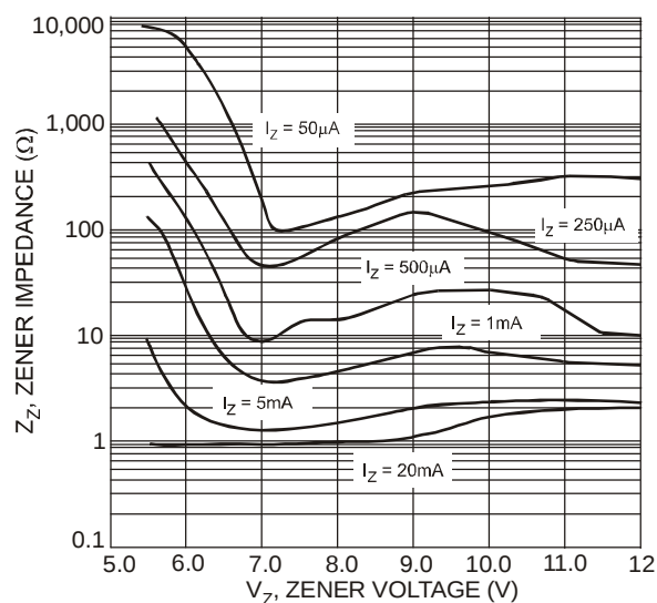
Fig. 11 Typical Zener Impedance Characteristics, DDZX5V6B - DDZX12C
