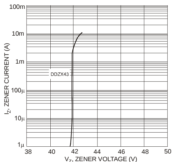
Fig. 9 Typical Zener Breakdown Characteristics, DDZX43
