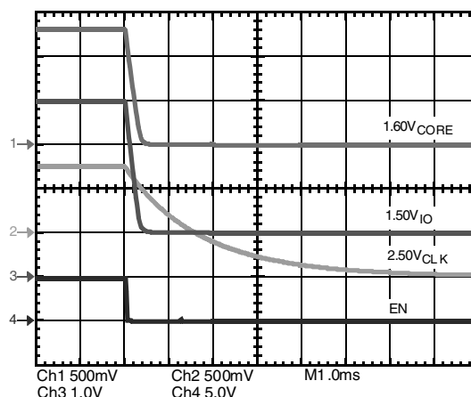
Figure 12. Shutdown Waveforms
