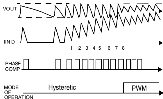
Figure 9. Hysteretic to PWM Transition
