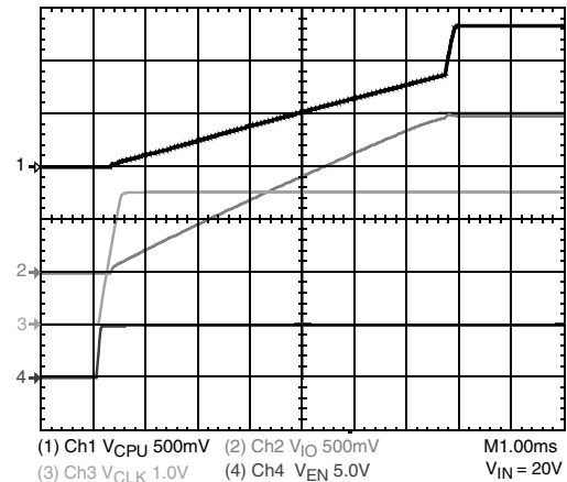
Figure 2. Initial Startup
