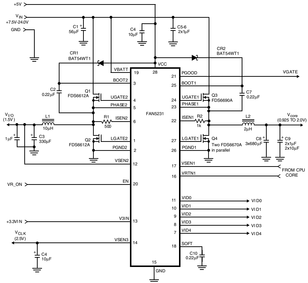
Figure 13. Application Circuit
