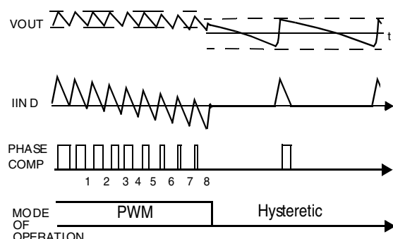
Figure 8. PWM to Hysteretic Transition
