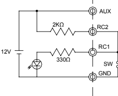
Using internal 12V auxiliary output
