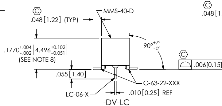
FIG 1 MMS-140-02-XXX-XV-LC SHOWN
