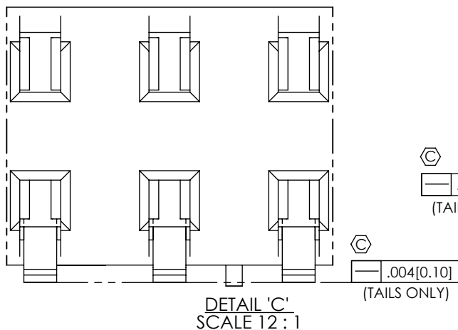
FIG 3 MMS-140-02-XXX-DH-LC SHOWN
