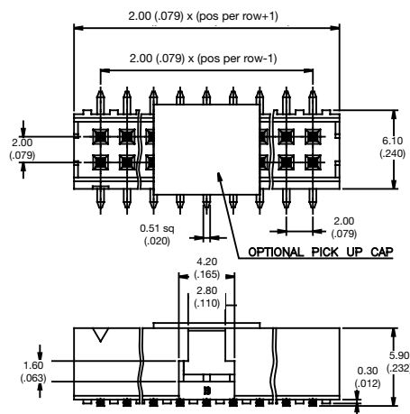
98424 Surface mount
