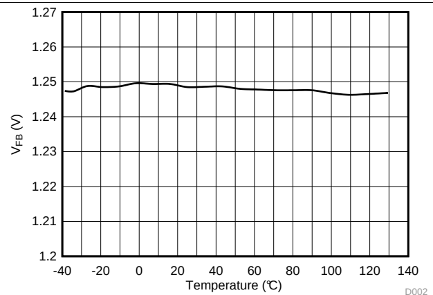
Figure 2. V_{FB} vs Temperature
