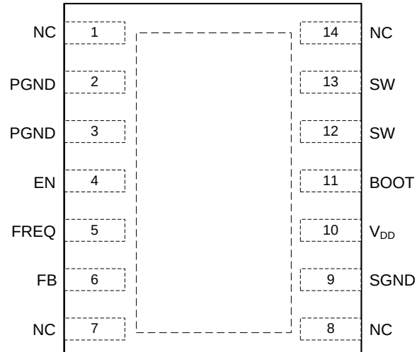
NHL Package 14-Pin WSON Top View
