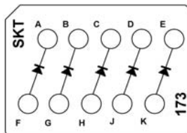
CTJ420E173 Five JANTX 1N5418 Diodes
