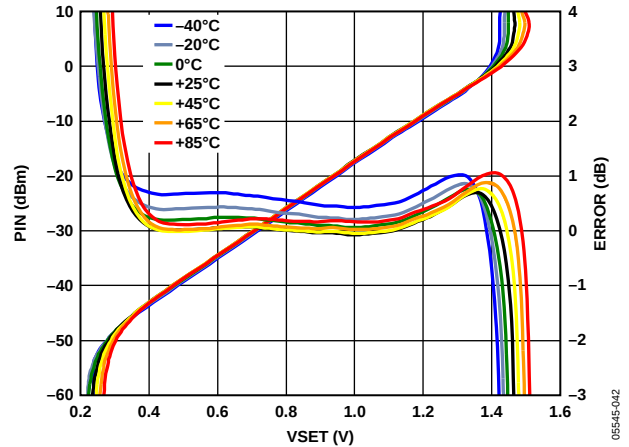
Figure 36. Typical Drift at 900 GHz for Various Temperatures
