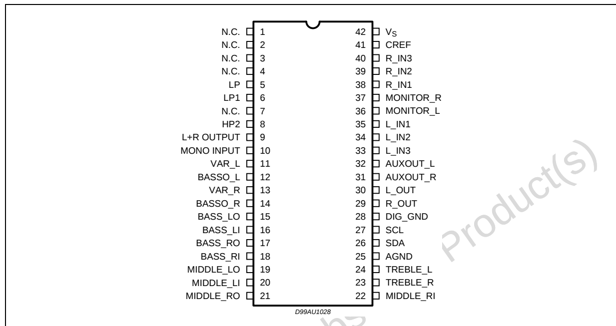
Figure 3. Pin Description
