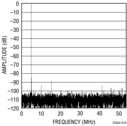
LTC2254: 8192 Point FFT, f_{IN} = 5\text{MHz} , -1\text{dB} , 2V Range, 105Mps
