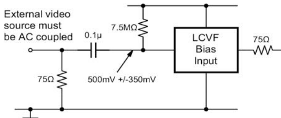
Figure 8. Biased SCART with DC-Coupled Outputs
