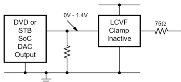
Figure 5. DC-Coupled Inputs and Outputs
