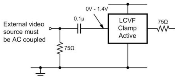
Figure 7. SCART with DC-Coupled Outputs
