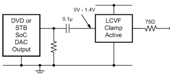
Figure 6. AC-Coupled Inputs, DC-Coupled Outputs
