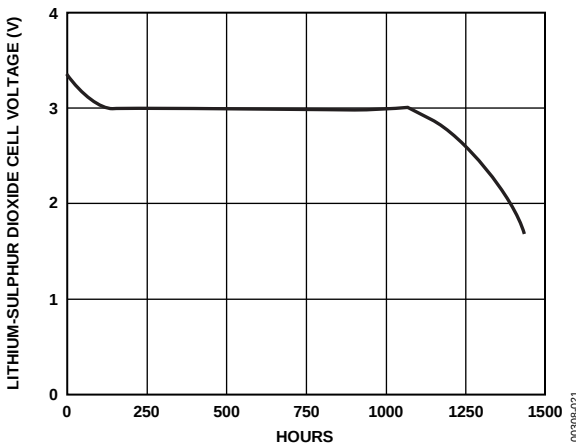
Figure 21. Lithium-Sulphur Dioxide Cell Discharge Characteristic with OP490 and 100 k \Omega Loads
