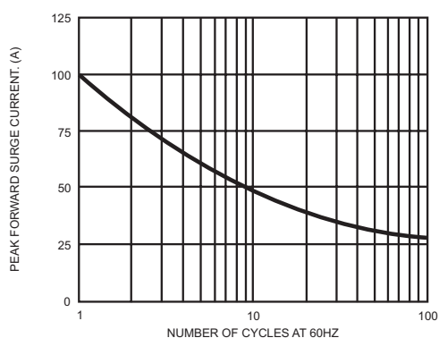
FIG.2- MAXIMUM NON-REPETITIVE FORWARD SURGE CURRENT
