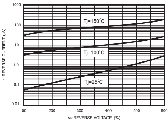
FIG.4- TYPICALS REVERSE CHARACTERISTICS
