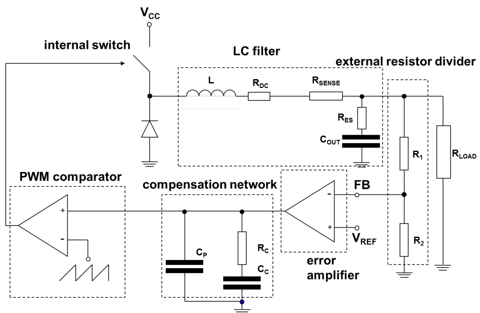
Figure 9. Constant current loop block diagramConstant current loop block diagram
