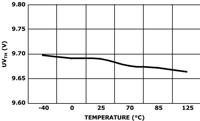
FIGURE 6. UV THRESHOLD
