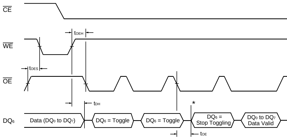
Figure 9 Data Polling during Embedded Algorithm Operation Timing Diagram
