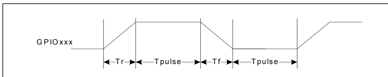
FIGURE 51-7: GPIO TIMING
