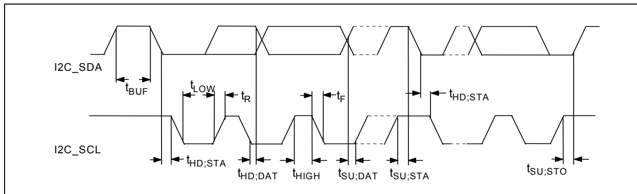
FIGURE 51-25: I2C/SMBUS TIMING
