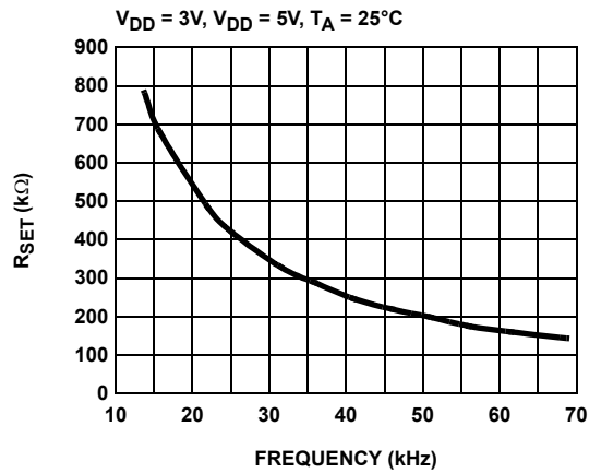
FIGURE 1. R_{SET} vs HORIZONTAL FREQUENCY
