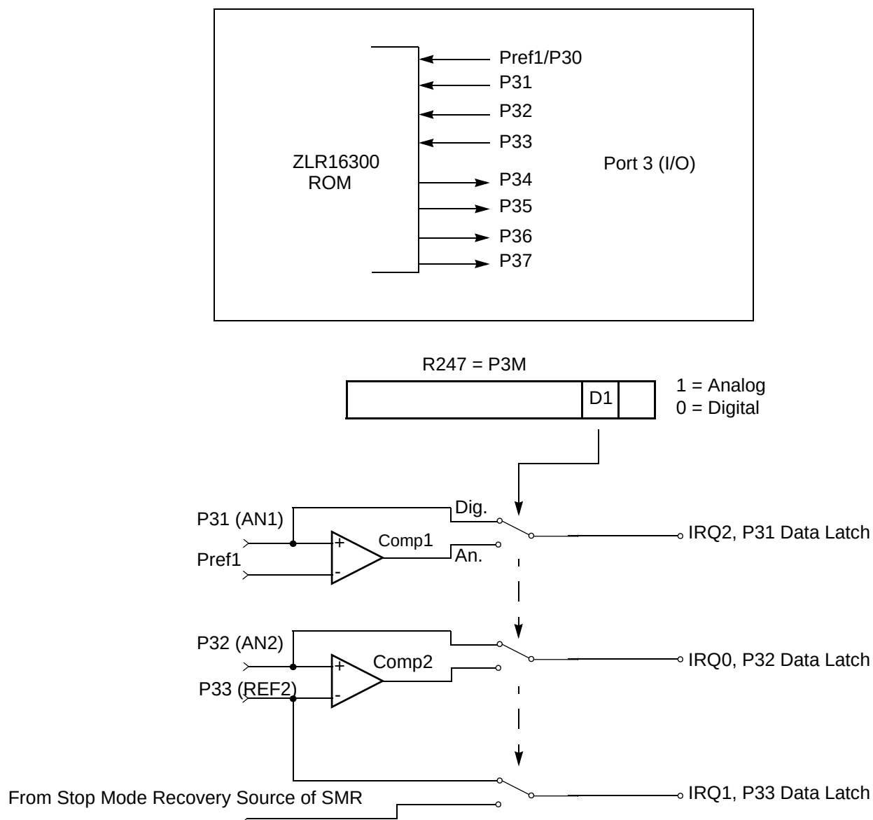
Figure 7. Port 3 Configuration
