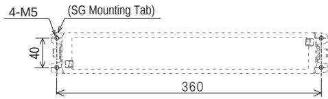
Figure 8. SG Type Mounting Hole Dimensions
