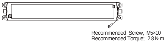
Figure 9. SG Type Installation
