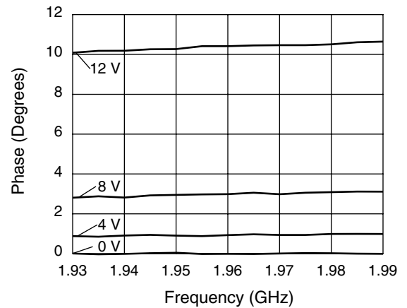
Phase vs. Frequency and Control Voltage — PCS Band
