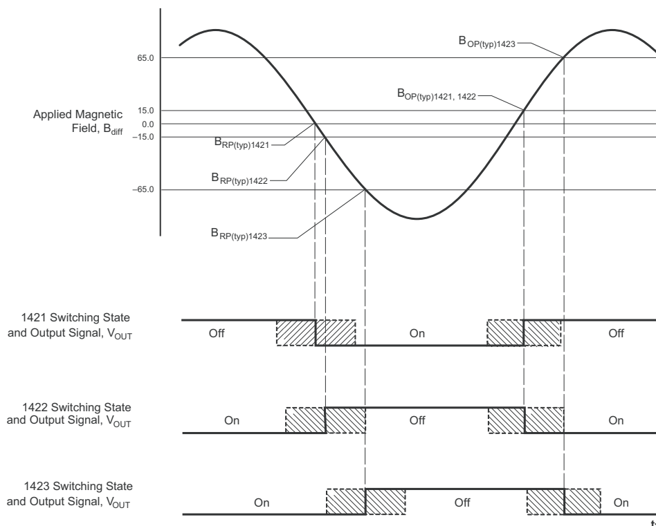
Figure 2. Comparative typical output characteristics. This chart illustrates the switch points and the output polarities of the A1421, A1422, and the A 1423. Characteristics shown without delay, see characteristic data charts for delay and phase shift contributions.
