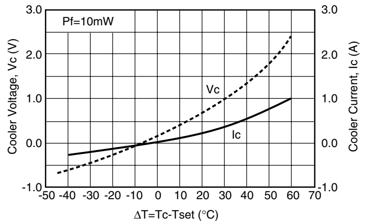
Fig. 4 Case Temperature Dependence of TEC Performance
