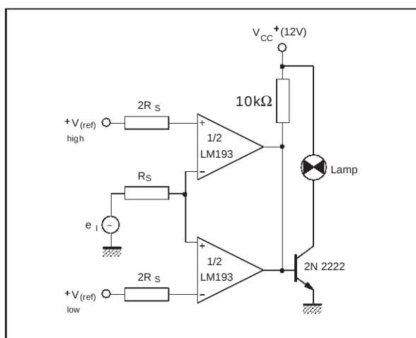
LIMIT COMPARATOR
