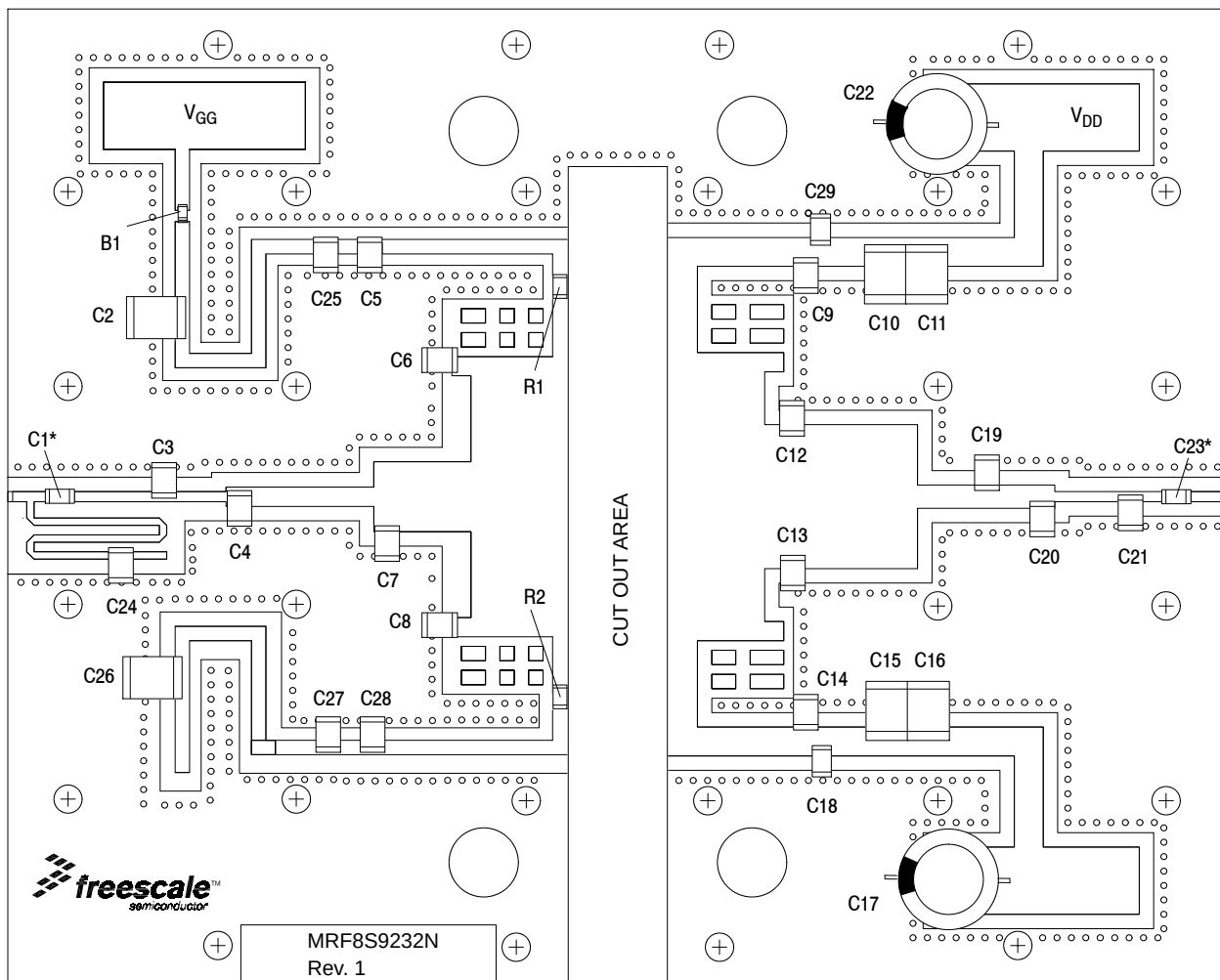
Figure 12. MRF8S9232NR3 Test Circuit Component Layout — 865-895 MHz
