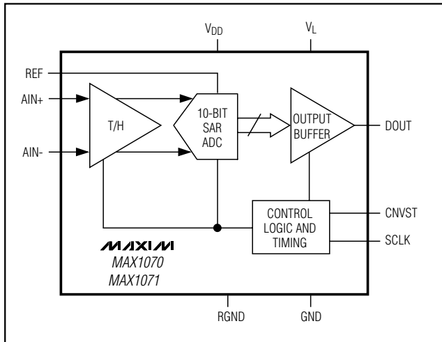
Figure 3. Functional Diagram
