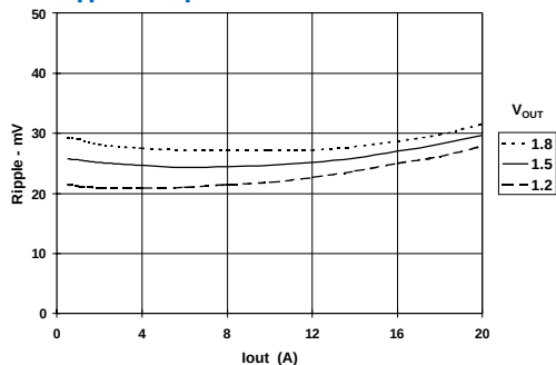
Ripple vs Output Current
